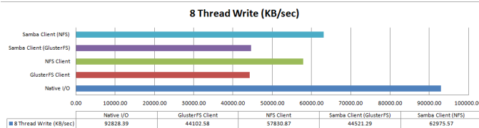
Figure 7 – 8 Thread Write
