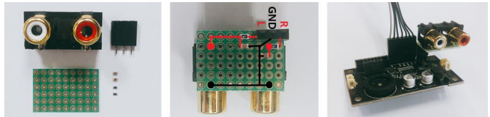
Figure 7 – Adding an RCA connector for line out to the Stereo Boom Bonnet
