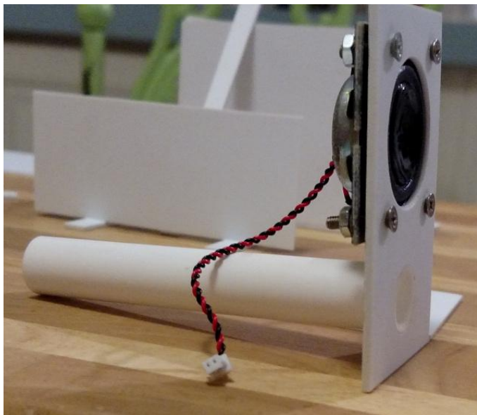
Figure 2 - Closeup of the tube attached
