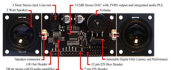
Figure 1 – Annotated diagram of the Stereo Boom Bonnet
