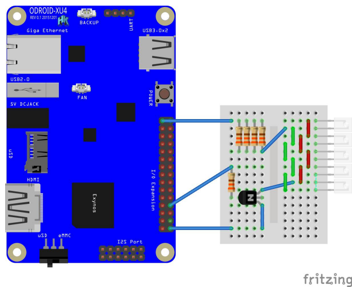
Figure 02 - fritzing breadboard view of IR blaster)
