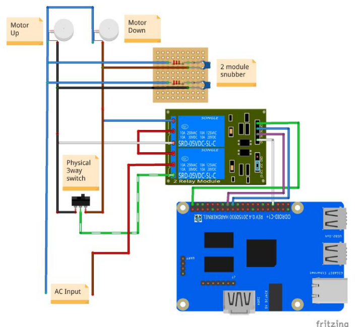
Figure 10 – Controlling a window blind motor
