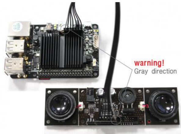
Figure 5 - Attaching the Stereo Boom Bonnet to an ODROID-C1+/C2
