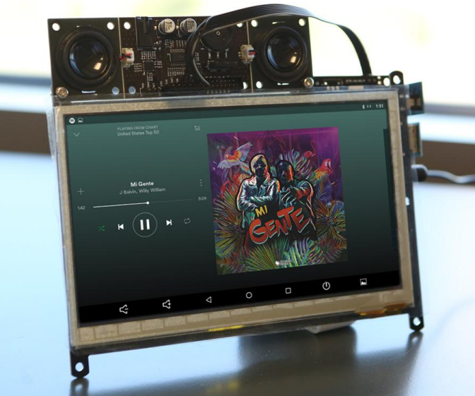
Figure 3 - The Stereo Boom Bonnet easily mounts to the ODROID-VU7
