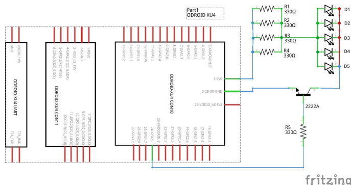
Figure 03 - Fritzing circuit diagram of IR blaster
