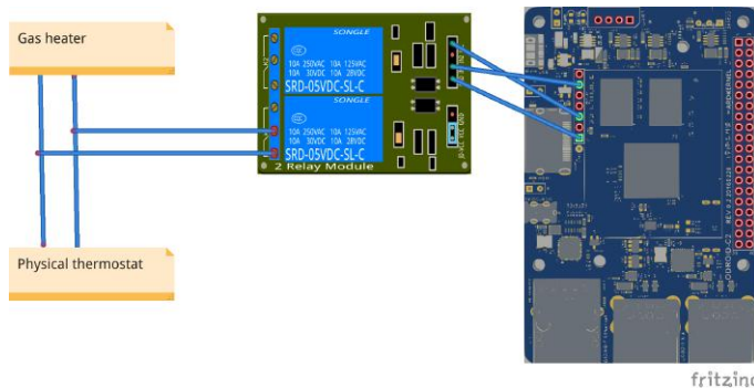
Figure 7 - Implementation details
