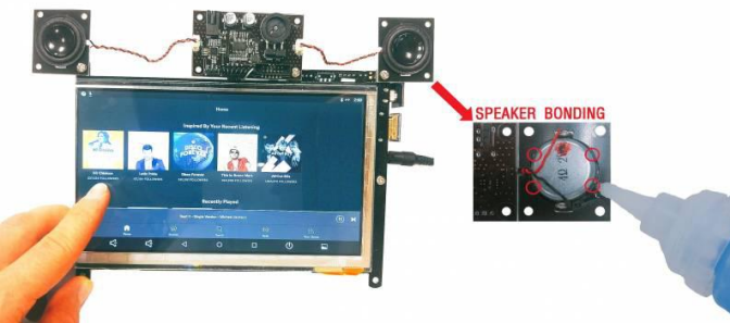
Figure 4 - The Stereo Boom Bonnet speakers can also be separated and attached anywhere with a small amount of glue
