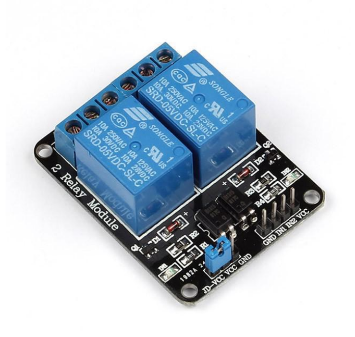
Figure 6 – SainSmart 2 Channel Relay
