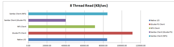
Figure 9 – 8 Thread Read
